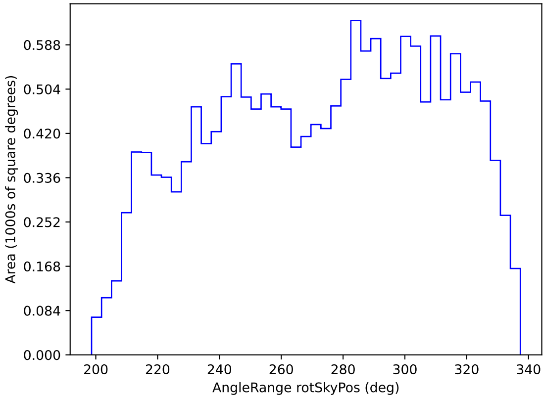
ddf_loaded_half_fl4_v3.4_10yrs WFD y band: AngleRange rotSkyPos
