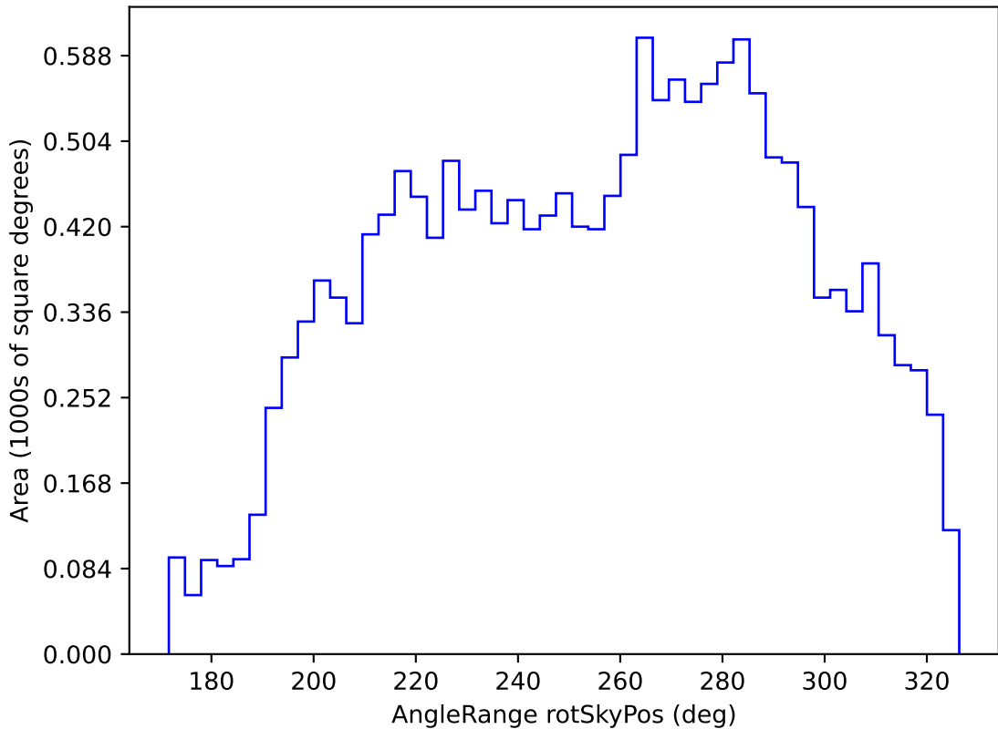
ddf_loaded_half_fl4_v3.4_10yrs WFD u band: AngleRange rotSkyPos
