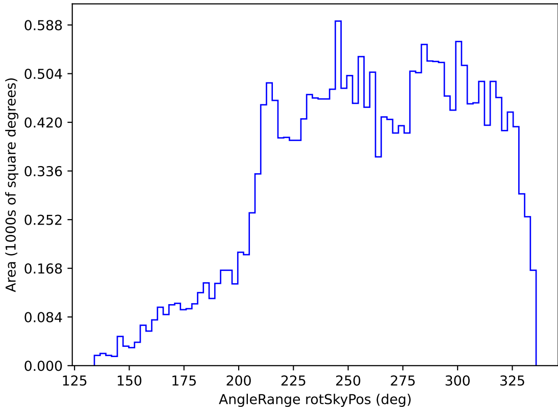
ddf_loaded_half_fl4_v3.4_10yrs All sky y band: AngleRange rotSkyPos
