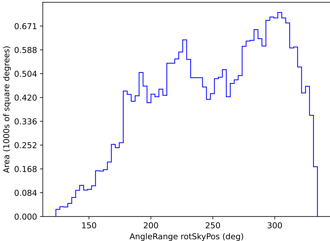
ddf_loaded_half_fl4_v3.4_10yrs All sky g band: AngleRange rotSkyPos
