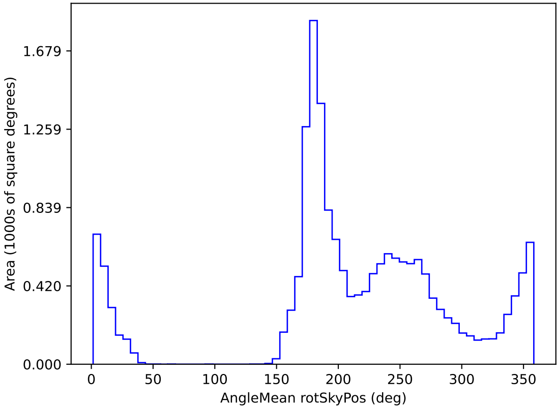
ddf_loaded_half_fl4_v3.4_10yrs WFD z band: AngleMean rotSkyPos
