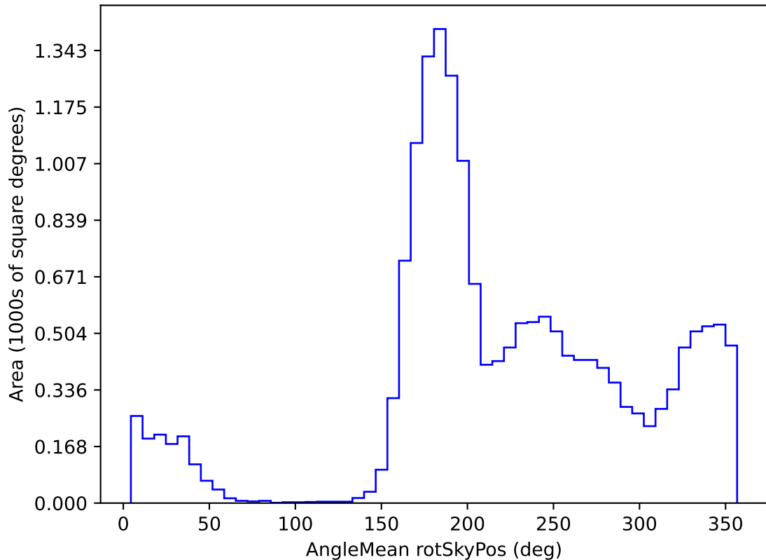
ddf_loaded_half_fl4_v3.4_10yrs WFD u band: AngleMean rotSkyPos
