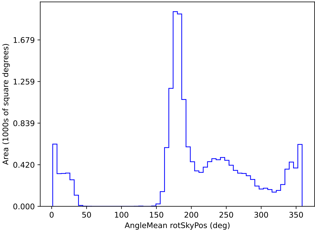
ddf_loaded_half_fl4_v3.4_10yrs WFD r band: AngleMean rotSkyPos
