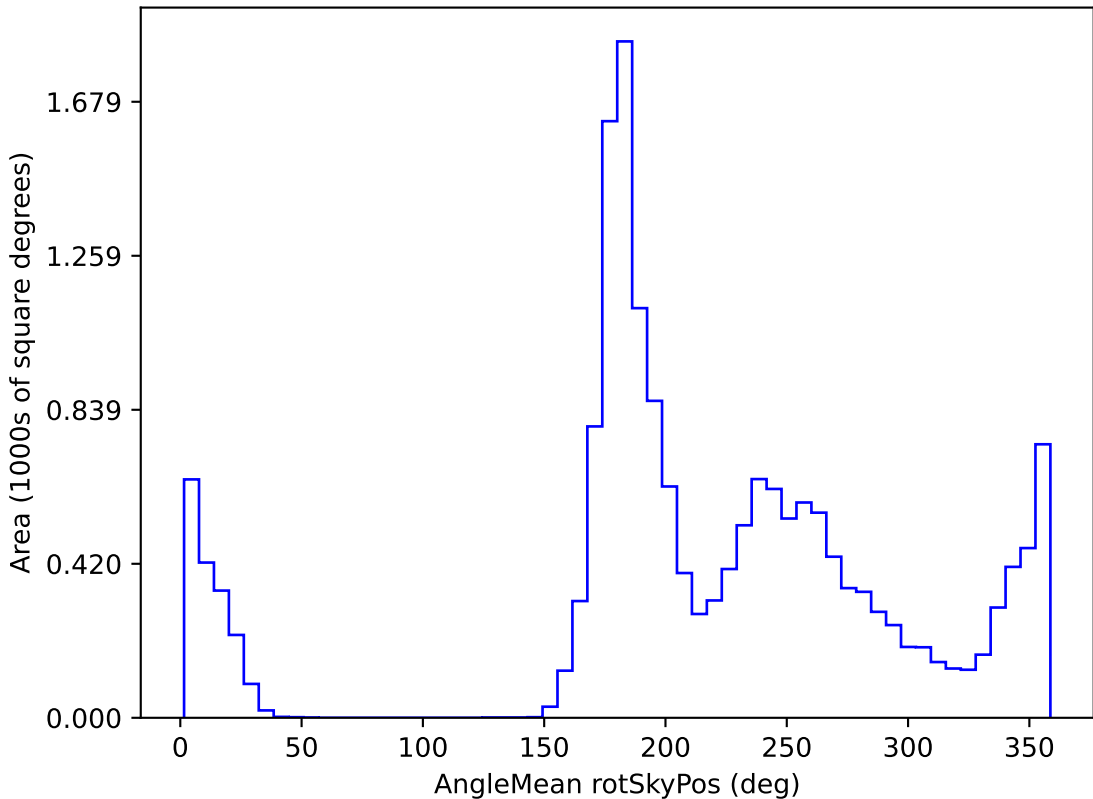
ddf_loaded_half_fl4_v3.4_10yrs WFD i band: AngleMean rotSkyPos
