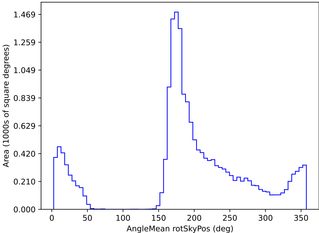
ddf_loaded_half_fl4_v3.4_10yrs WFD g band: AngleMean rotSkyPos
