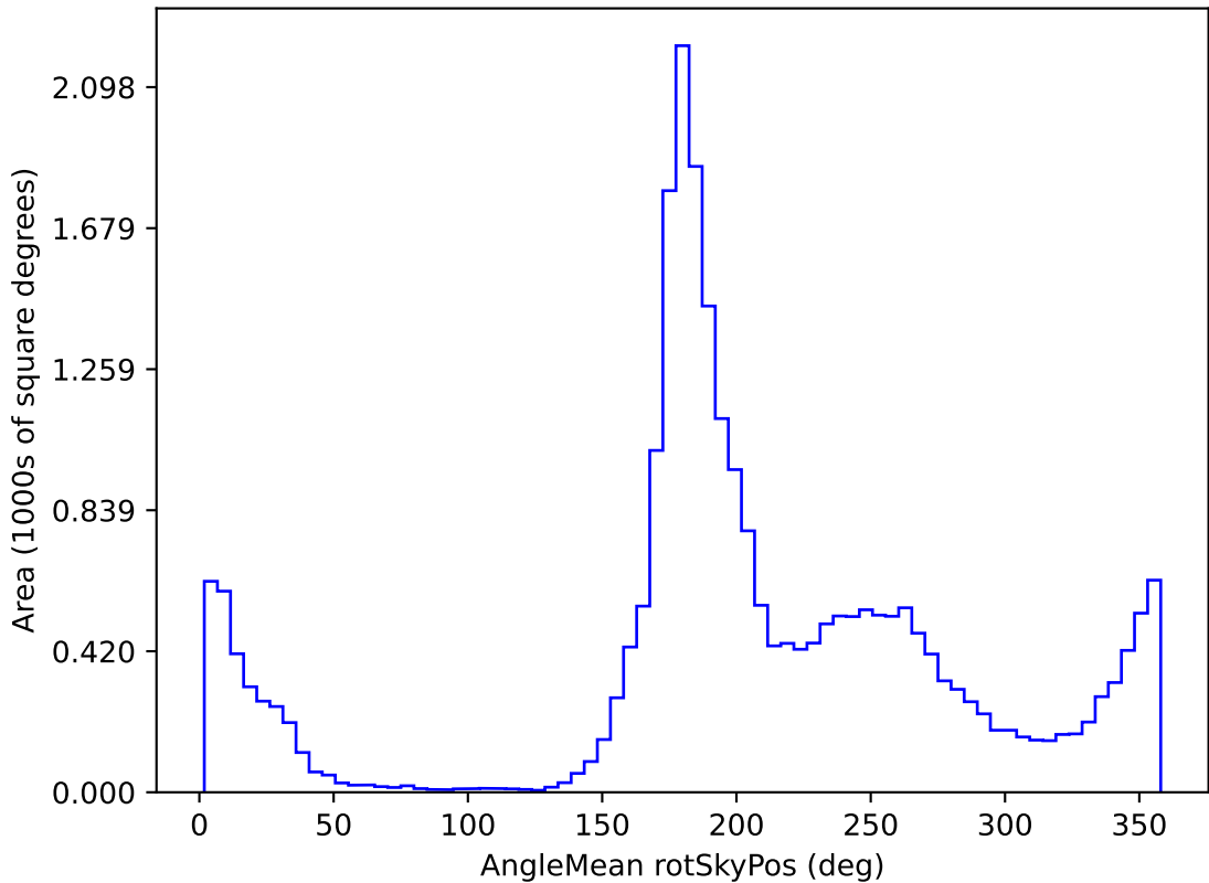
ddf_loaded_half_fl4_v3.4_10yrs All sky z band: AngleMean rotSkyPos
