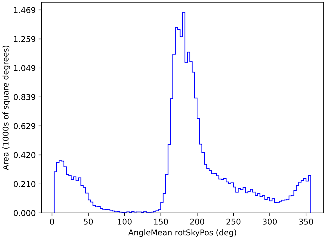
ddf_loaded_half_fl4_v3.4_10yrs All sky g band: AngleMean rotSkyPos
