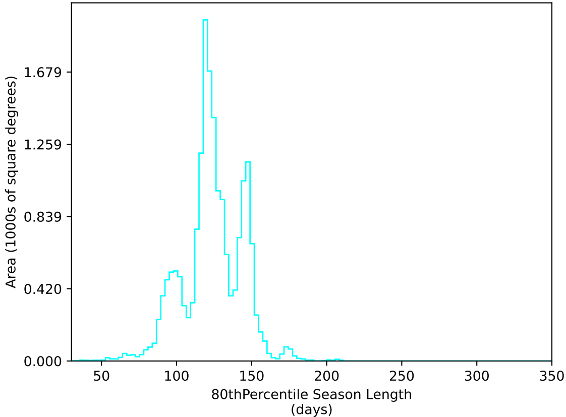
ddf_loaded_half_fl4_v3.4_10yrs WFD u band: 80thPercentile Season Length
