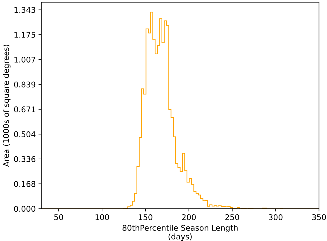
ddf_loaded_half_fl4_v3.4_10yrs WFD r band: 80thPercentile Season Length
