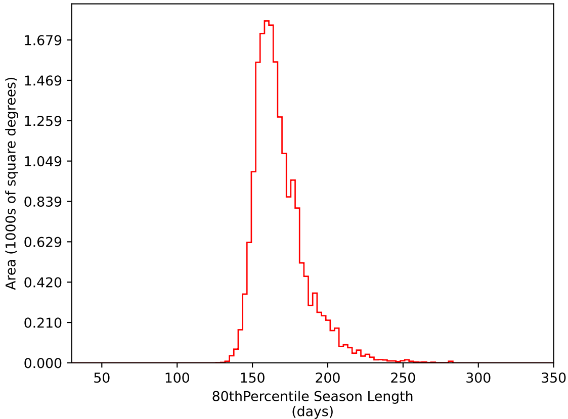
ddf_loaded_half_fl4_v3.4_10yrs WFD i band: 80thPercentile Season Length
