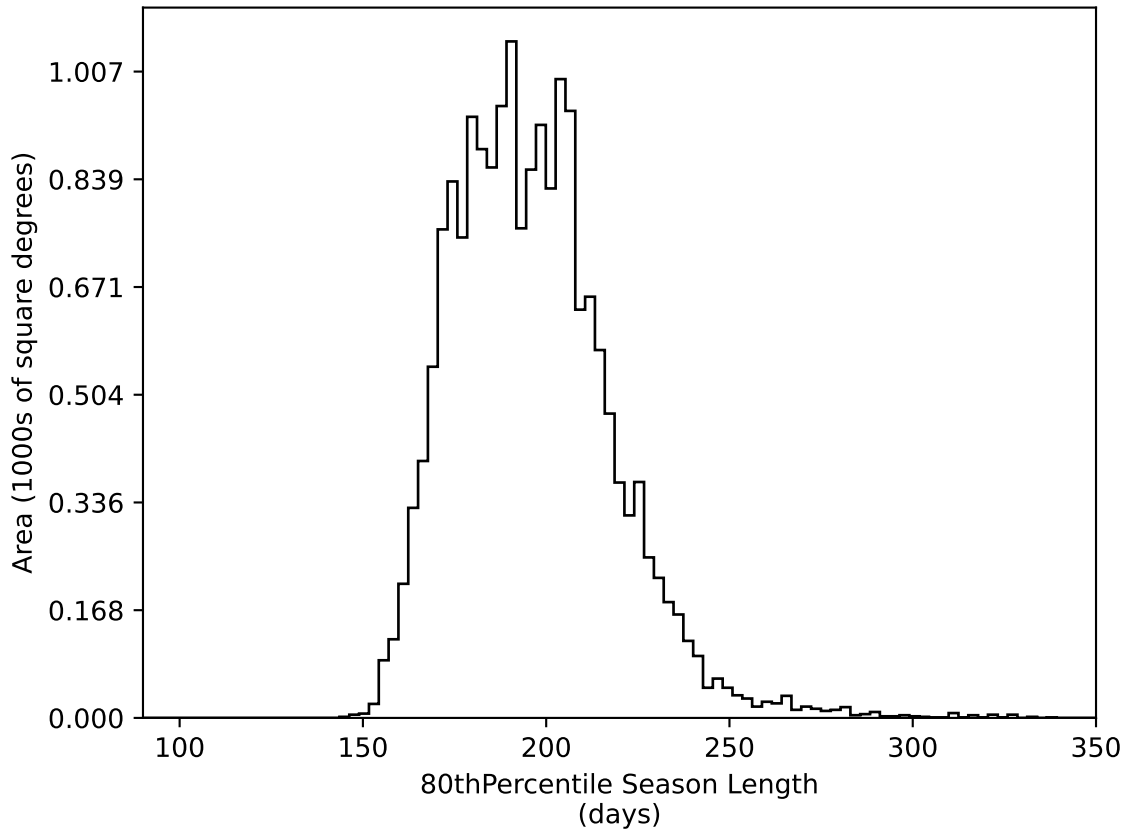
ddf_loaded_half_fl4_v3.4_10yrs WFD all bands: 80thPercentile Season Length
