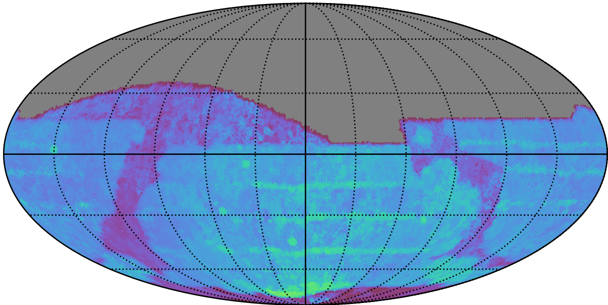
ddf_loaded_half_fl4_v3.4_10yrs All sky z band: 80thPercentile Season Length
