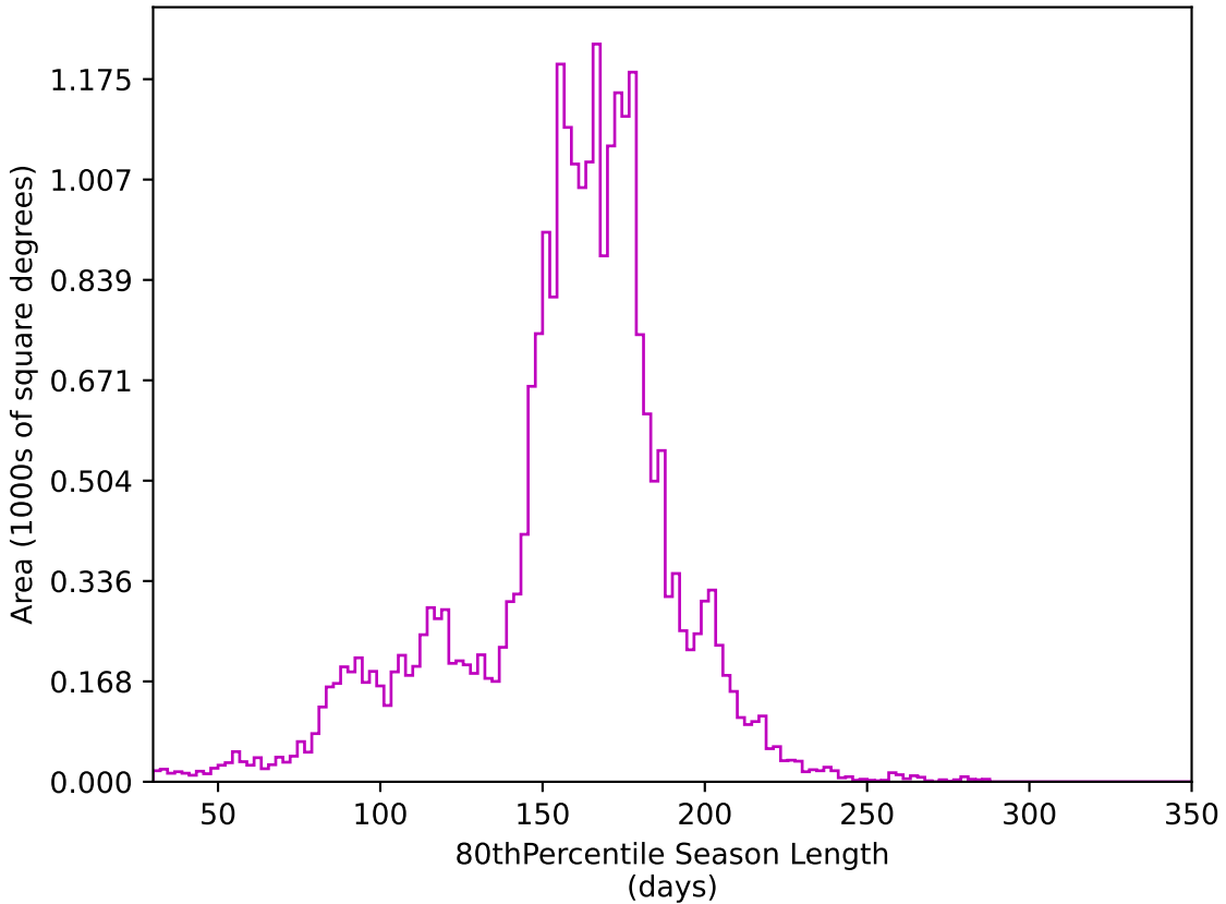
ddf_loaded_half_fl4_v3.4_10yrs All sky z band: 80thPercentile Season Length
