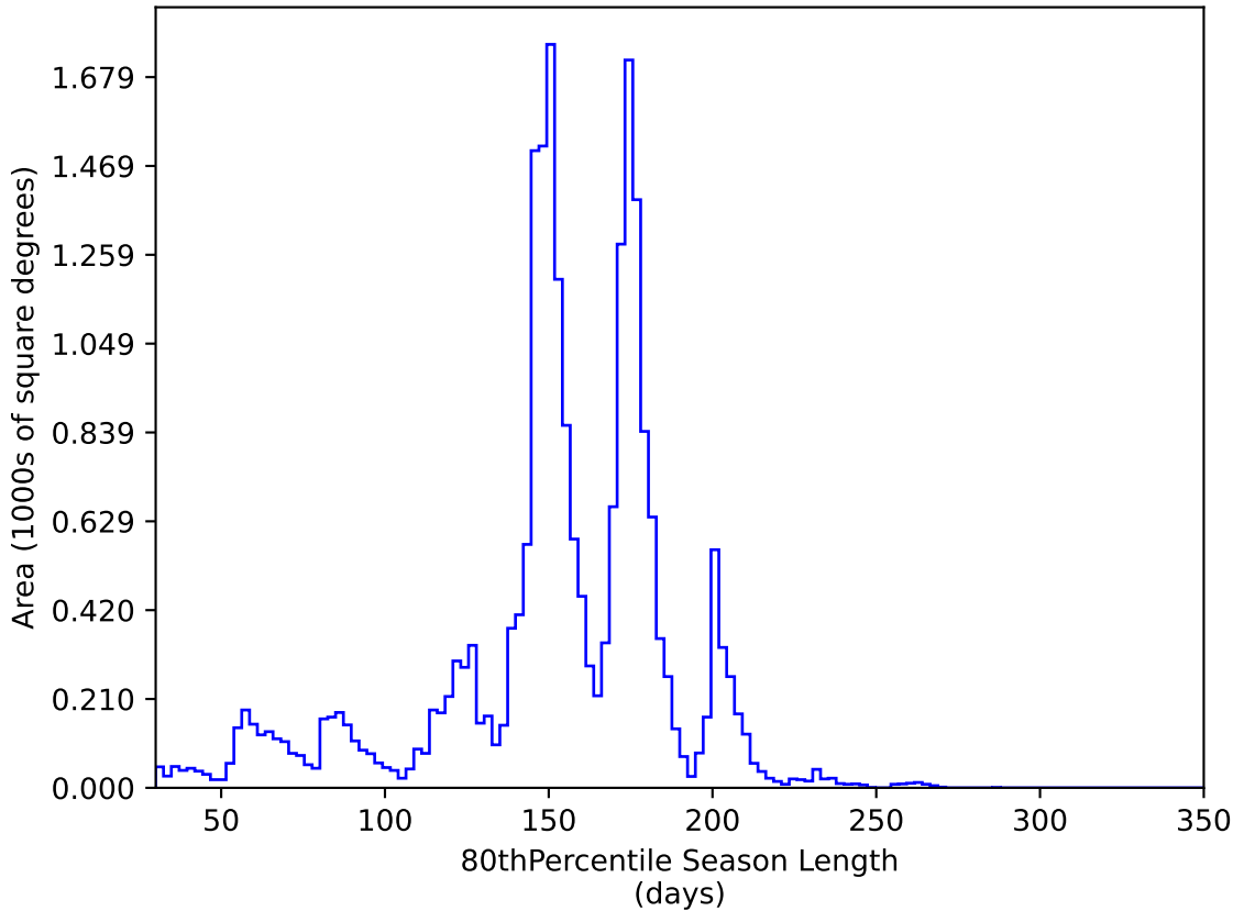
ddf_loaded_half_fl4_v3.4_10yrs All sky y band: 80thPercentile Season Length
