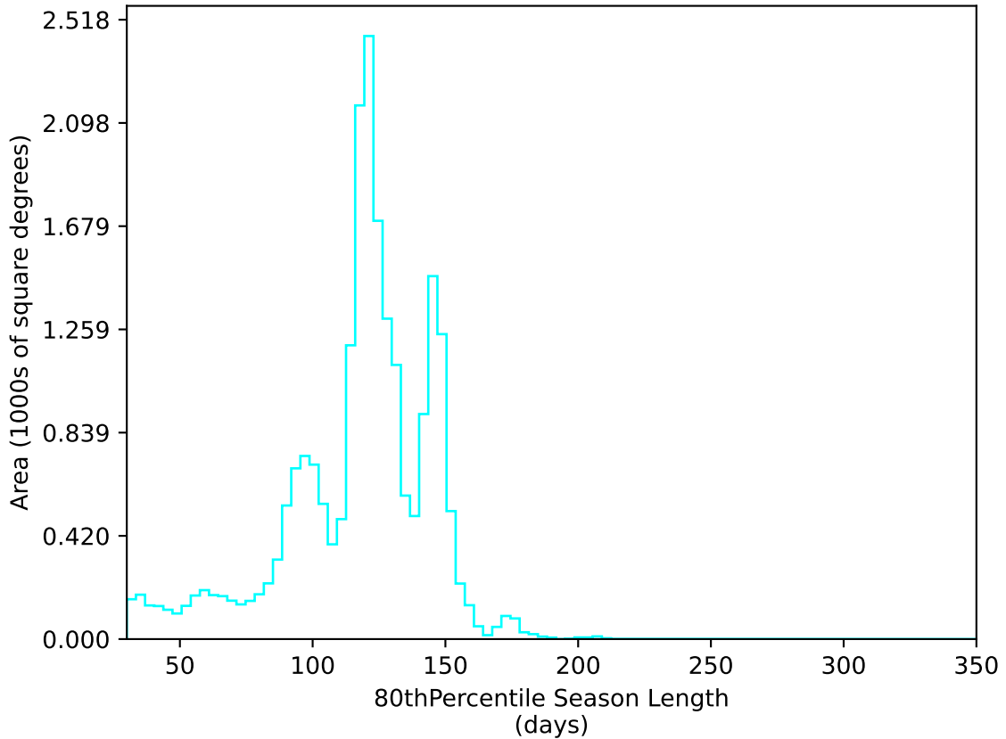
ddf_loaded_half_fl4_v3.4_10yrs All sky u band: 80thPercentile Season Length
