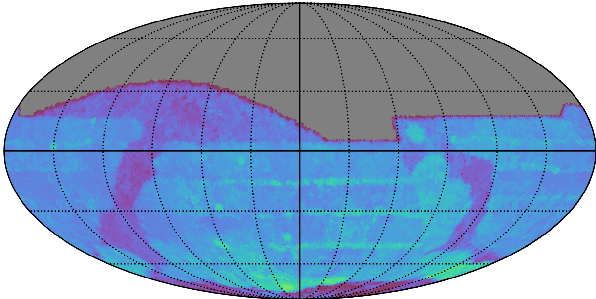
ddf_loaded_half_fl4_v3.4_10yrs All sky r band: 80thPercentile Season Length
