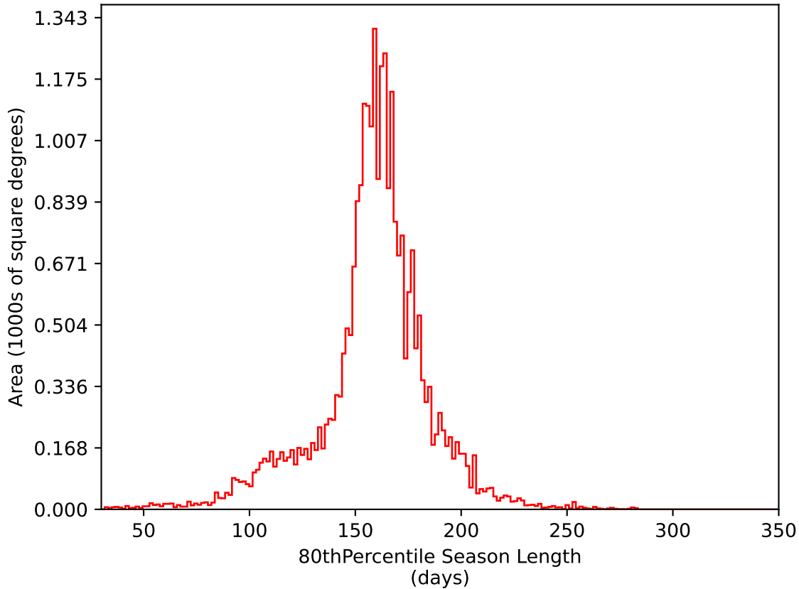
ddf_loaded_half_fl4_v3.4_10yrs All sky i band: 80thPercentile Season Length
