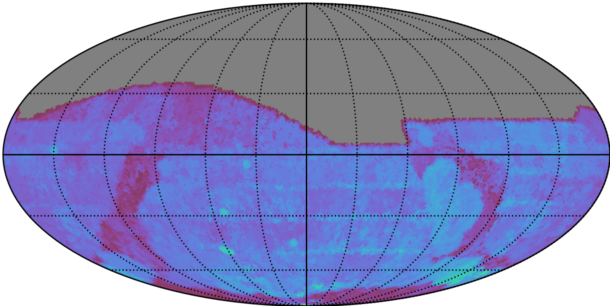
ddf_loaded_half_fl4_v3.4_10yrs All sky g band: 80thPercentile Season Length
