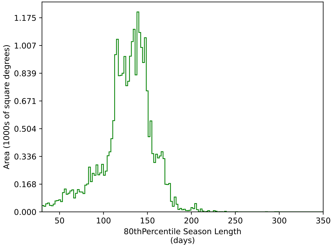
ddf_loaded_half_fl4_v3.4_10yrs All sky g band: 80thPercentile Season Length
