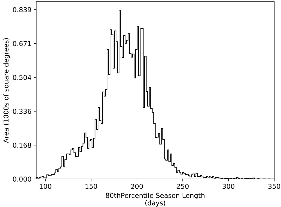
ddf_loaded_half_fl4_v3.4_10yrs All sky all bands: 80thPercentile Season Length
