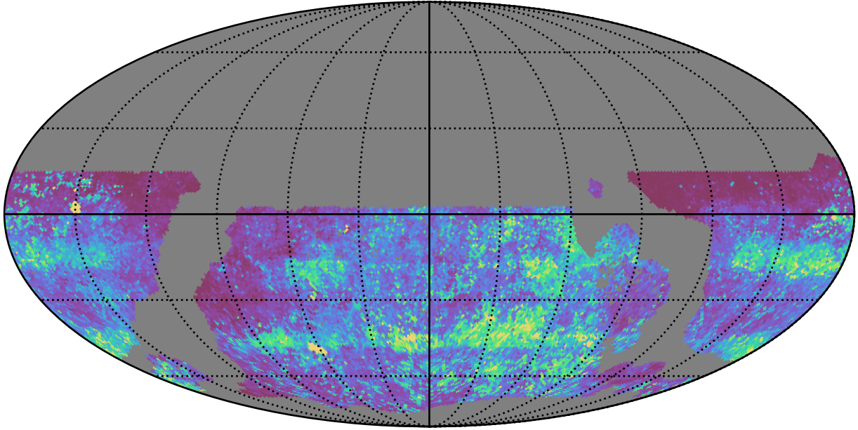
ddf_loaded_half_fl4_v3.4_10yrs WFD zy bands: 75th Percentile Intranight Timespan
