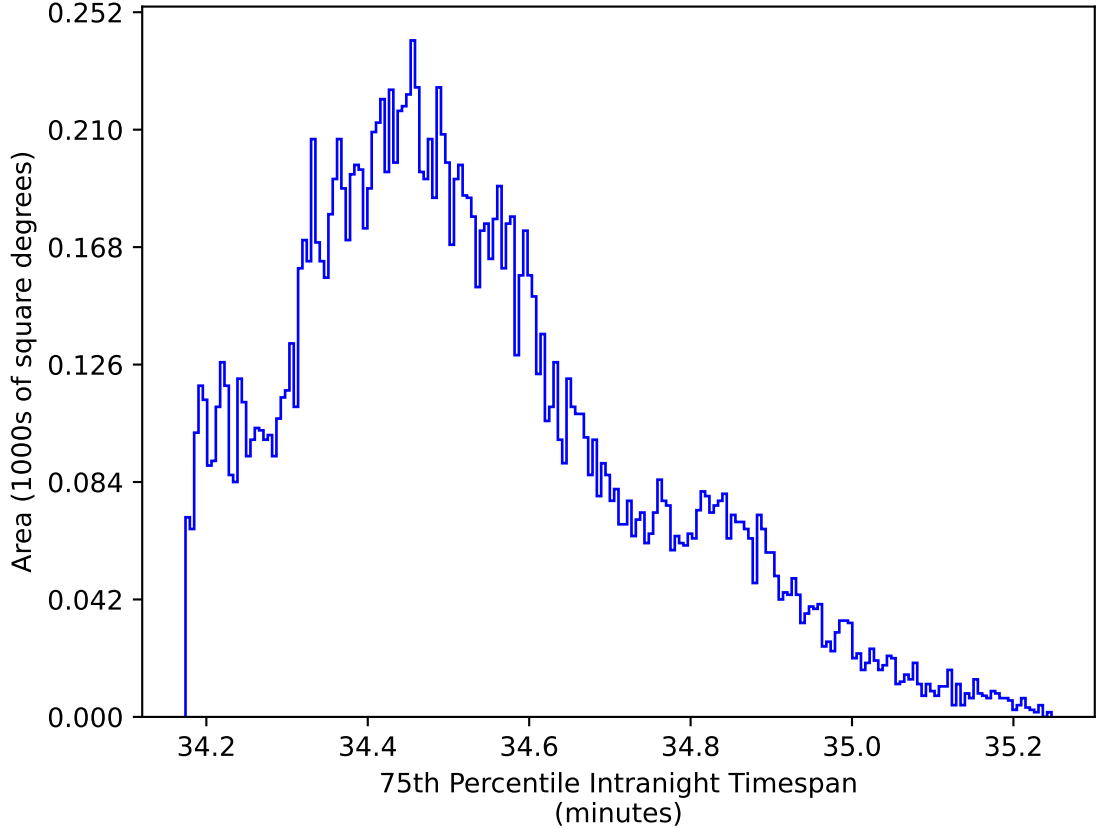
ddf_loaded_half_fl4_v3.4_10yrs WFD zy bands: 75th Percentile Intranight Timespan
