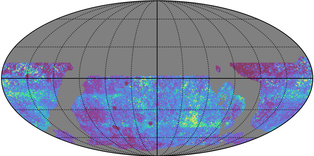
ddf_loaded_half_fl4_v3.4_10yrs WFD y band: 75th Percentile Intranight Timespan
