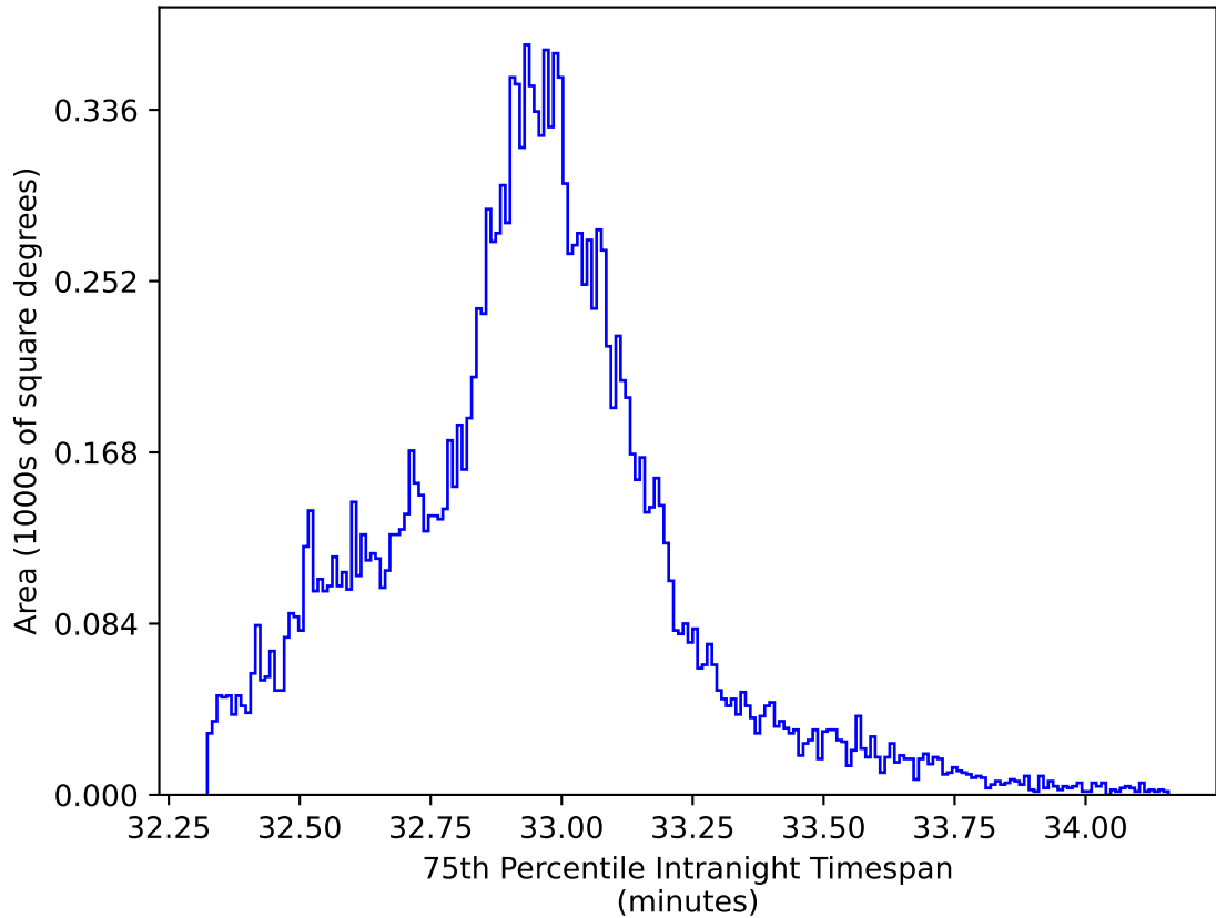
ddf_loaded_half_fl4_v3.4_10yrs WFD y band: 75th Percentile Intranight Timespan
