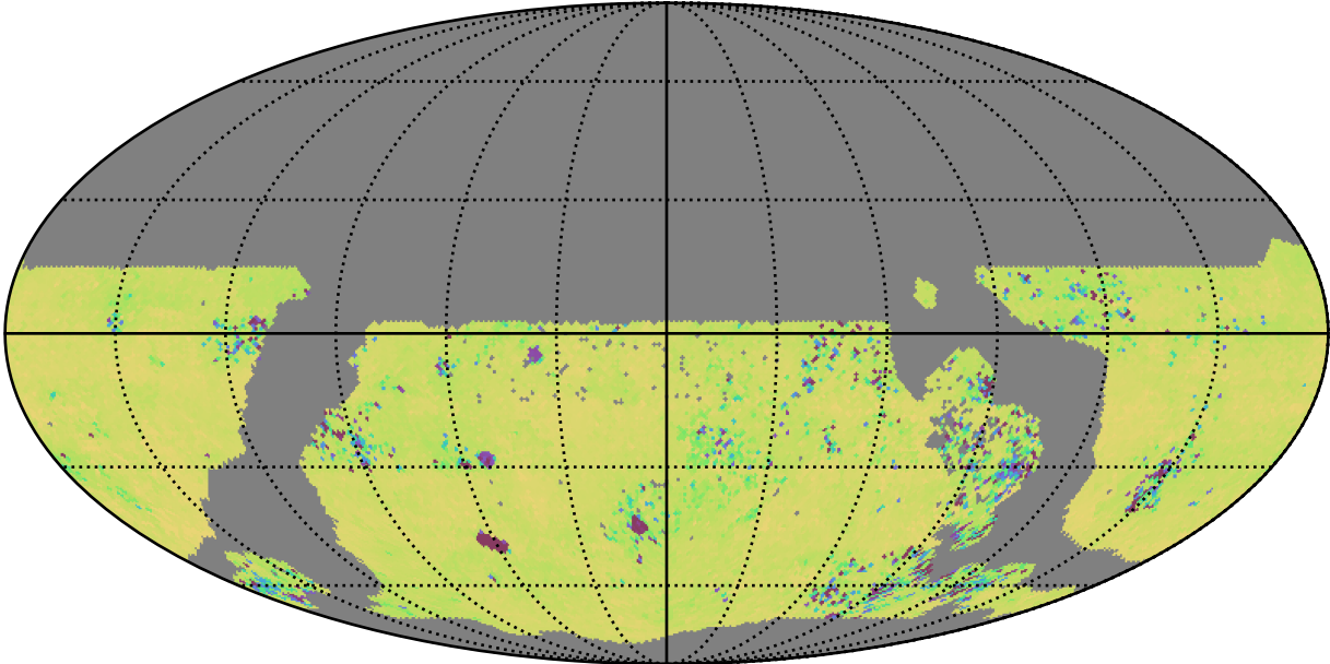
ddf_loaded_half_fl4_v3.4_10yrs WFD ug bands: 75th Percentile Intranight Timespan
