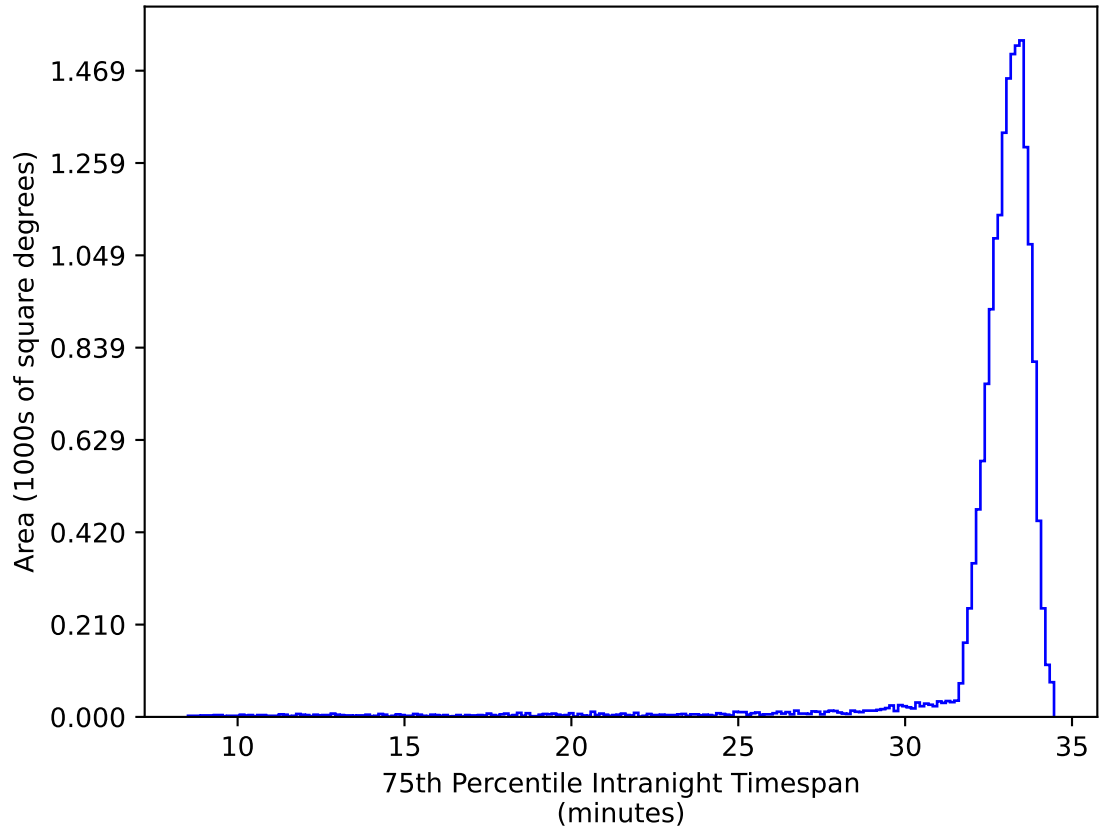
ddf_loaded_half_fl4_v3.4_10yrs WFD ug bands: 75th Percentile Intranight Timespan
