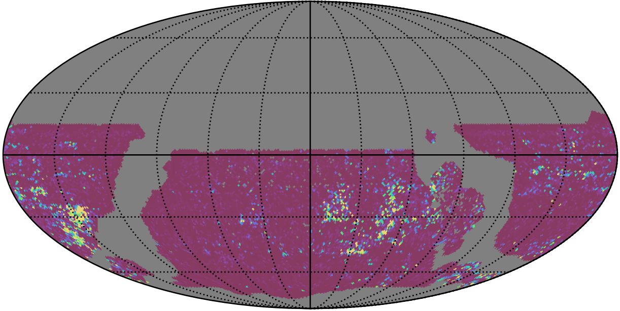
ddf_loaded_half_fl4_v3.4_10yrs WFD u band: 75th Percentile Intranight Timespan
