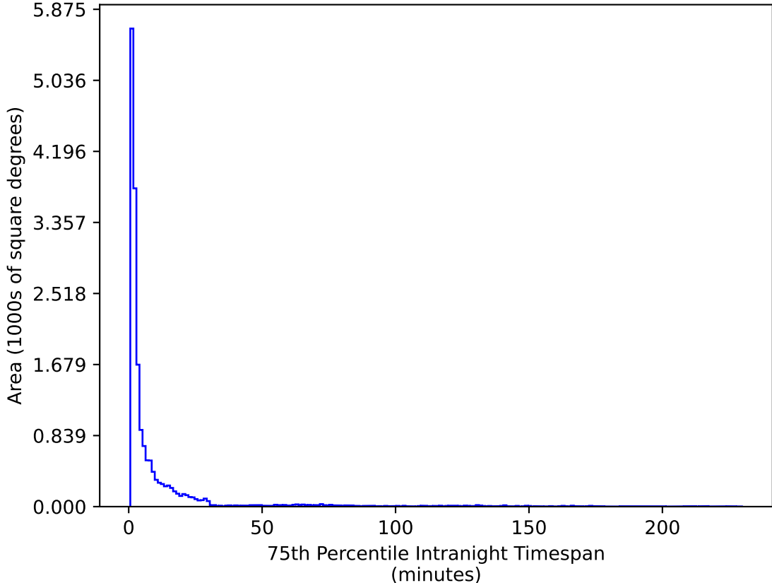
ddf_loaded_half_fl4_v3.4_10yrs WFD u band: 75th Percentile Intranight Timespan
