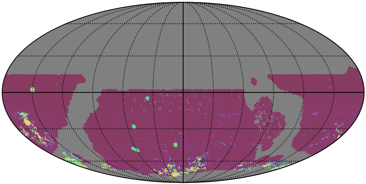
ddf_loaded_half_fl4_v3.4_10yrs WFD ri bands: 75th Percentile Intranight Timespan
