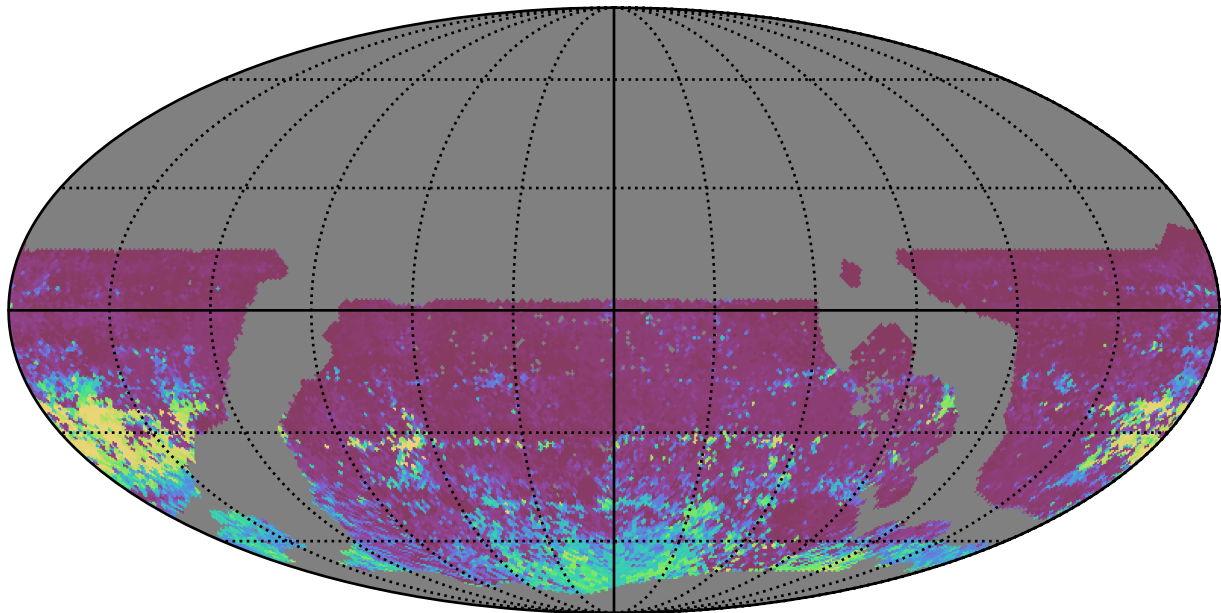
ddf_loaded_half_fl4_v3.4_10yrs WFD r band: 75th Percentile Intranight Timespan
