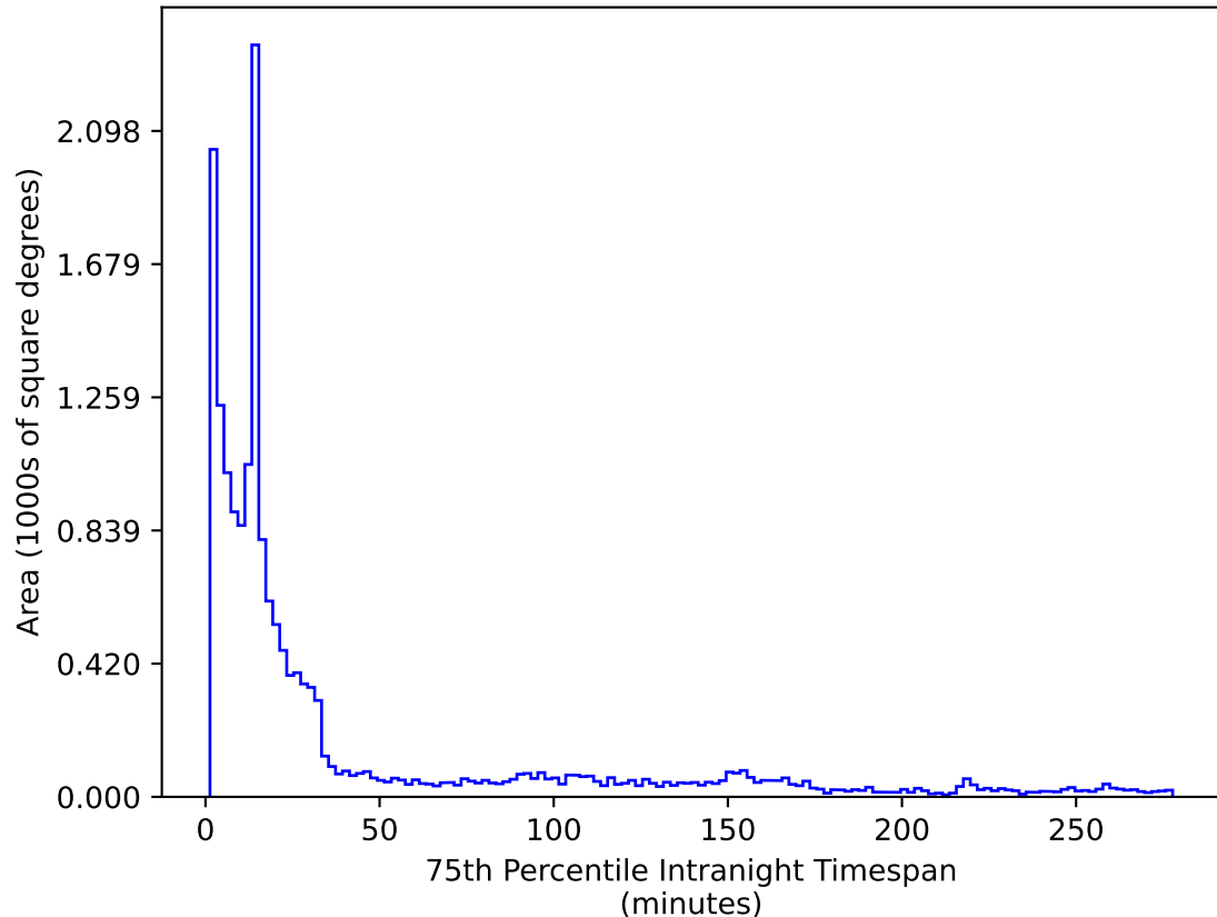
ddf_loaded_half_fl4_v3.4_10yrs WFD r band: 75th Percentile Intranight Timespan
