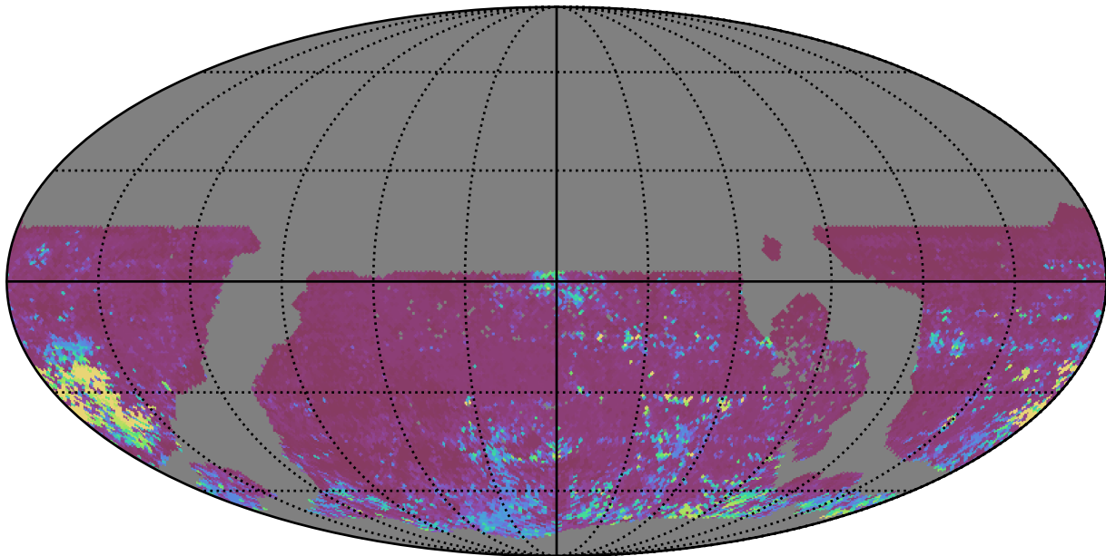
ddf_loaded_half_fl4_v3.4_10yrs WFD i band: 75th Percentile Intranight Timespan
