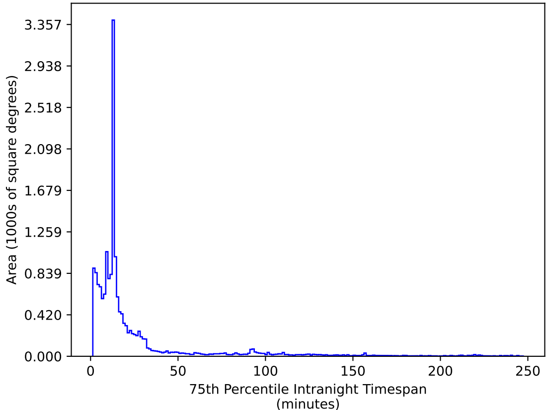
ddf_loaded_half_fl4_v3.4_10yrs WFD i band: 75th Percentile Intranight Timespan
