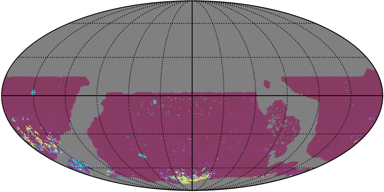
ddf_loaded_half_fl4_v3.4_10yrs WFD gr bands: 75th Percentile Intranight Timespan
