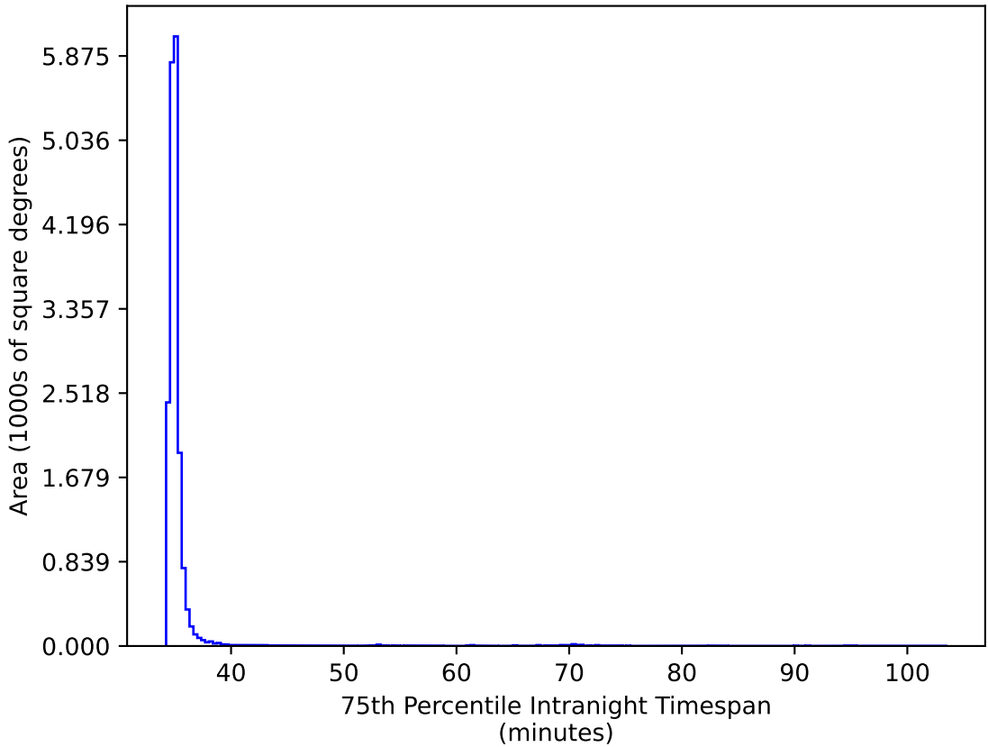
ddf_loaded_half_fl4_v3.4_10yrs WFD gr bands: 75th Percentile Intranight Timespan
