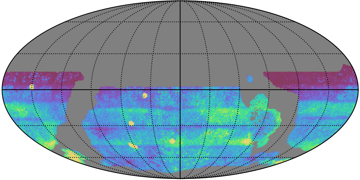
ddf_loaded_half_fl4_v3.4_10yrs WFD all bands: 75th Percentile Intranight Timespan
