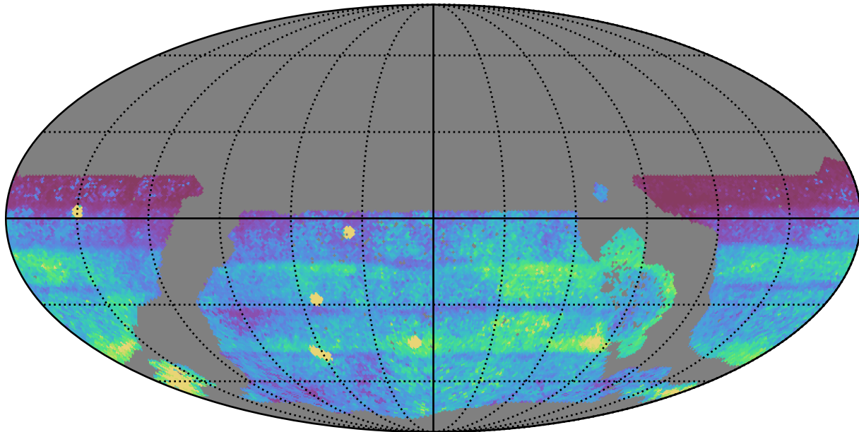
ddf_loaded_half_fl4_v3.4_10yrs WFD: 75th Percentile Intranight Timespan
