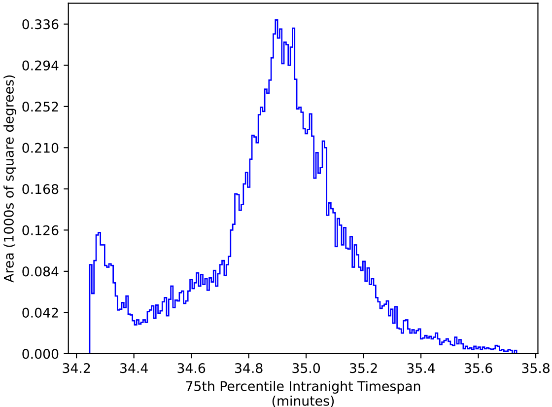
ddf_loaded_half_fl4_v3.4_10yrs WFD: 75th Percentile Intranight Timespan
