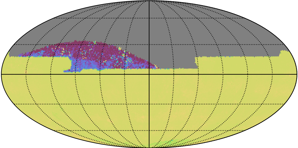
ddf_loaded_half_fl4_v3.4_10yrs All sky zy bands: 75th Percentile Intranight Timespan
