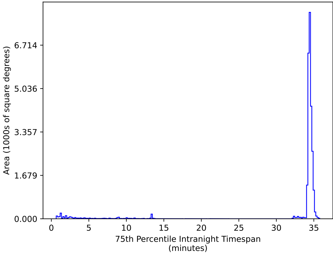
ddf_loaded_half_fl4_v3.4_10yrs All sky zy bands: 75th Percentile Intranight Timespan
