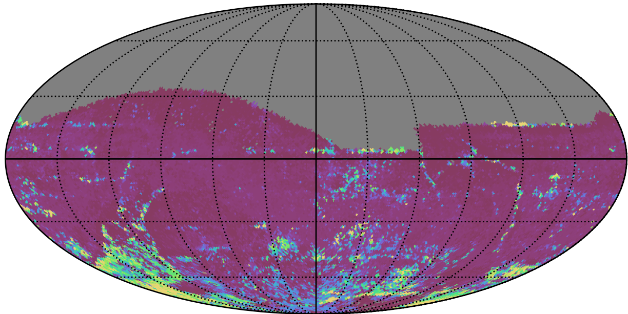
ddf_loaded_half_fl4_v3.4_10yrs All sky z band: 75th Percentile Intranight Timespan
