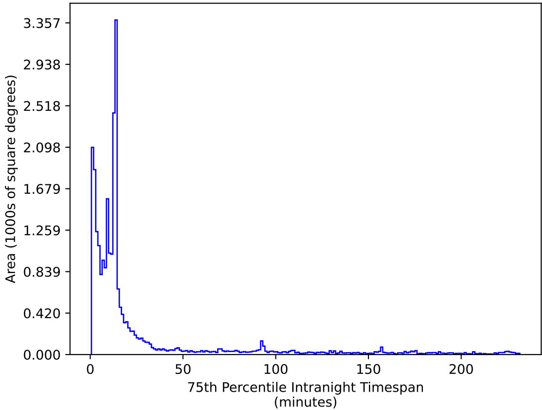
ddf_loaded_half_fl4_v3.4_10yrs All sky z band: 75th Percentile Intranight Timespan
