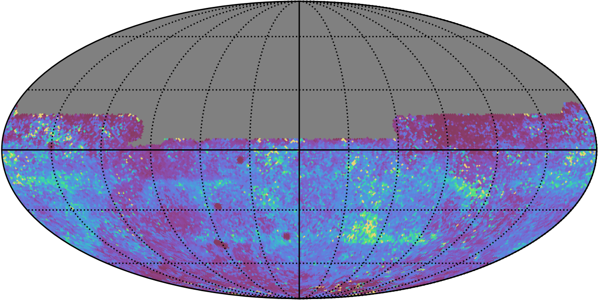
ddf_loaded_half_fl4_v3.4_10yrs All sky y band: 75th Percentile Intranight Timespan
