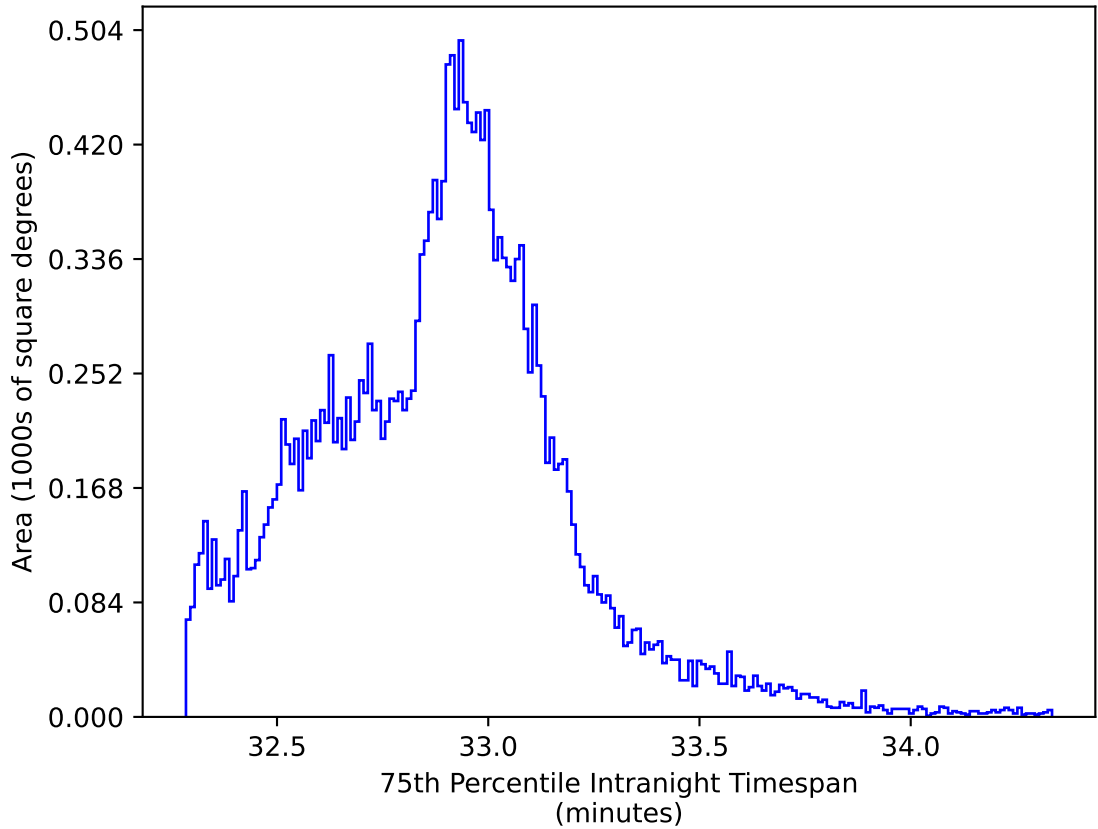
ddf_loaded_half_fl4_v3.4_10yrs All sky y band: 75th Percentile Intranight Timespan
