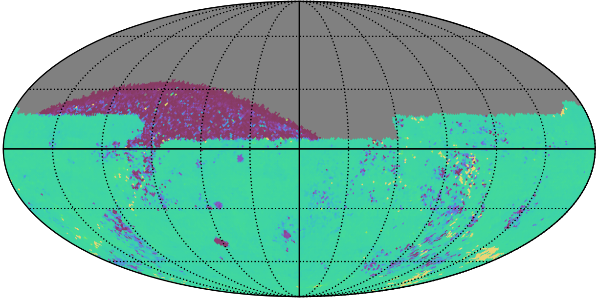
ddf_loaded_half_fl4_v3.4_10yrs All sky ug bands: 75th Percentile Intranight Timespan
