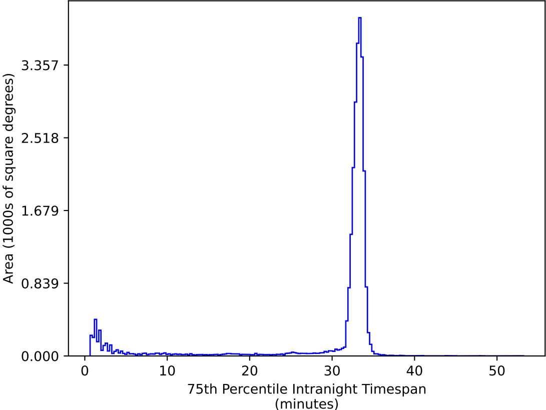
ddf_loaded_half_fl4_v3.4_10yrs All sky ug bands: 75th Percentile Intranight Timespan
